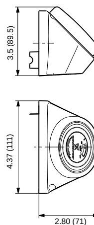
Fig. 13 Timer dimensions, current version
